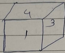
General (sum = 7 of two sides) Dice
